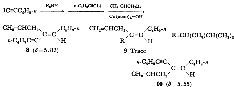
Scheme 4.
